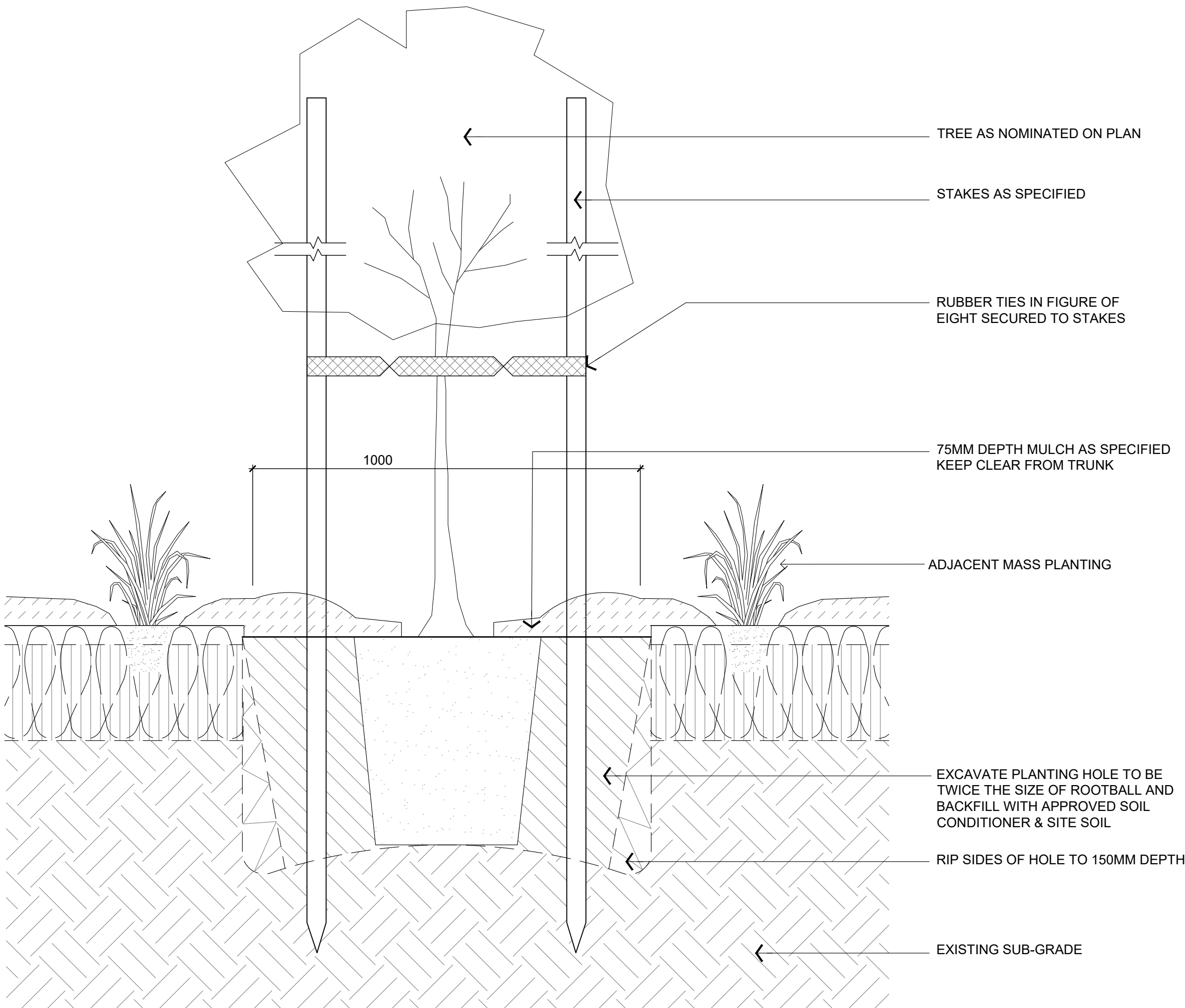
02 TREE PLANTING TYPICAL SECTION 1:10 SCALE
