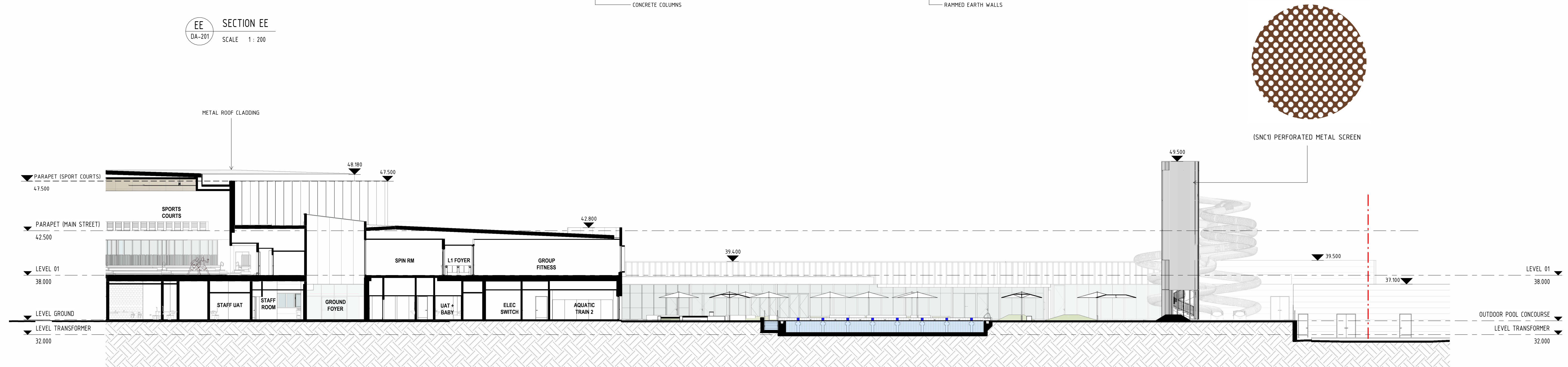
FF SECTION FF DA-201 SCALE 1:200
