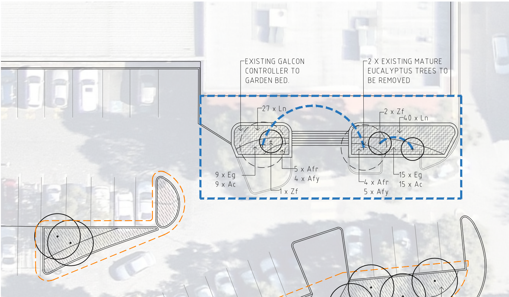
01 PLANTING PLAN - ENTRY AND PARKING ISLANDS 301 PLAN 1:250 @ A1
